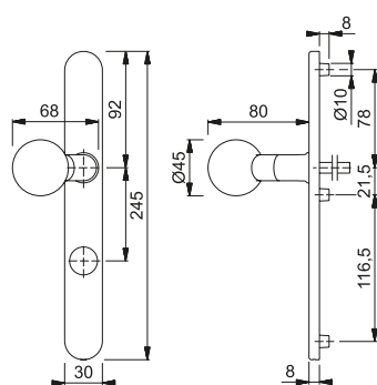
bouton E50G
