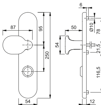
bouton FS-86G
