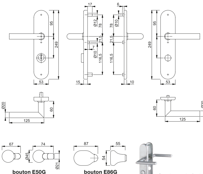
bouton E50G
