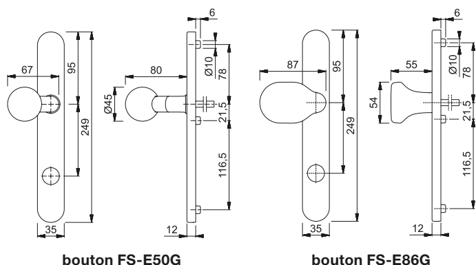
bouton FS-E50G
