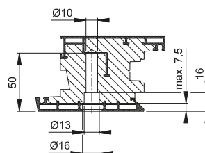
profile Pural
