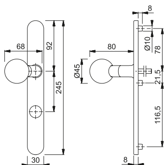
bouton FS-E50G
