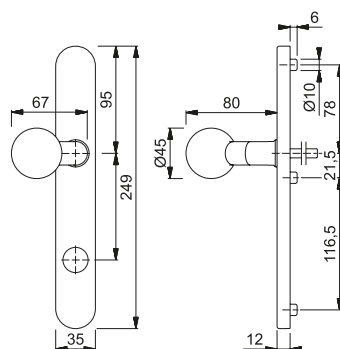
bouton FS-E50G
