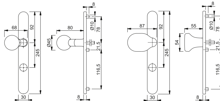
bouton E50G
