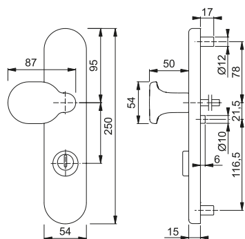
bouton FS-86G
