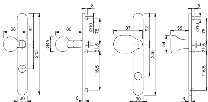
bouton FS-E50G
