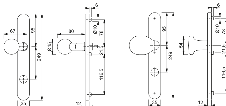
bouton E50G
